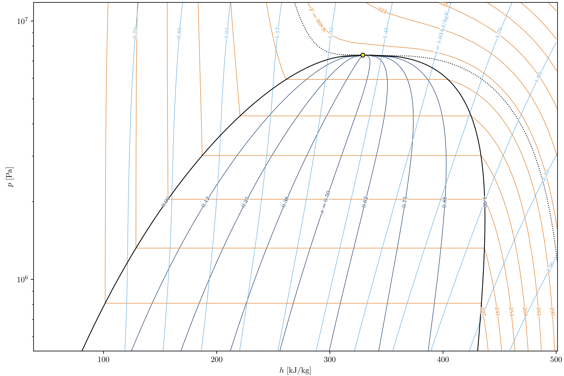
Thermodynamic Diagram (PH) – CO2
